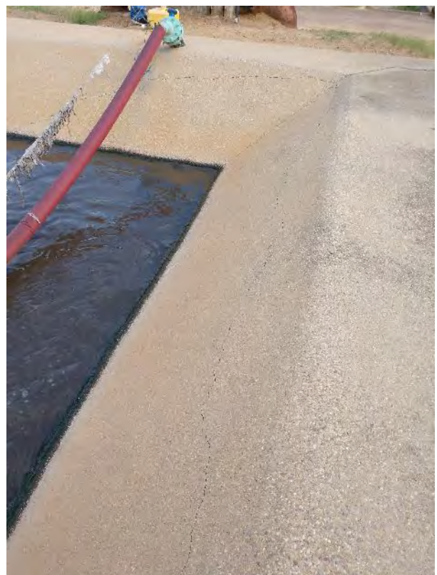
Figure 1.8: Cracking along northeast corner of Basin
